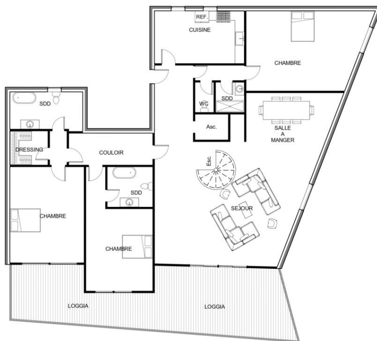
LOWER FLOOR
