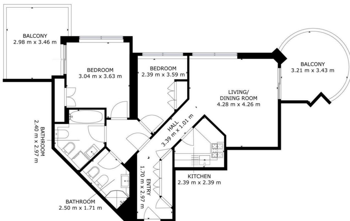
FLOOR 1
